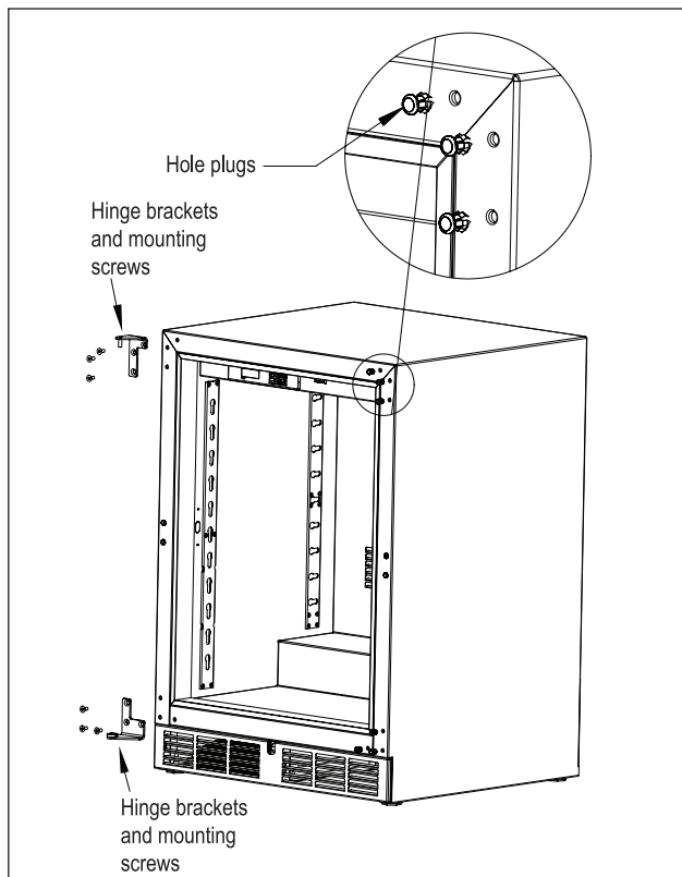
Figure 8. Hinge Removal
