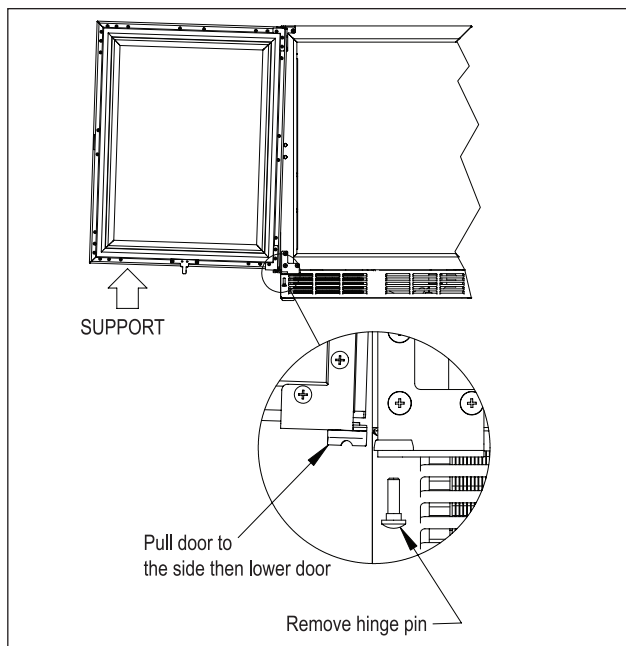
Figure 7. Door Removal
