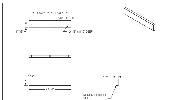
Figure 18. Wine Rack Trim, 15" models
