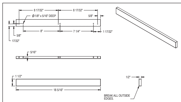
Figure 19. Wine Rack Trim, 24" models
