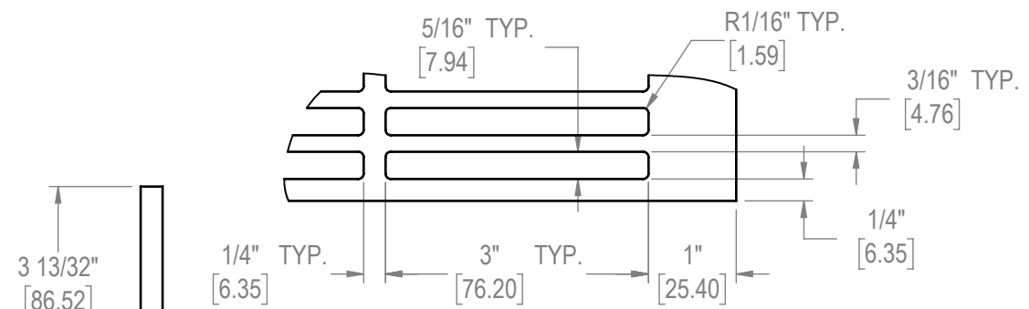
DETAIL C SCALE 1:2
